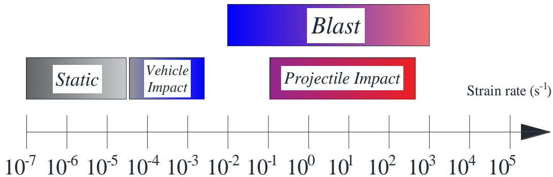
Figure 2: Loading rate range (Ekström 2015)
