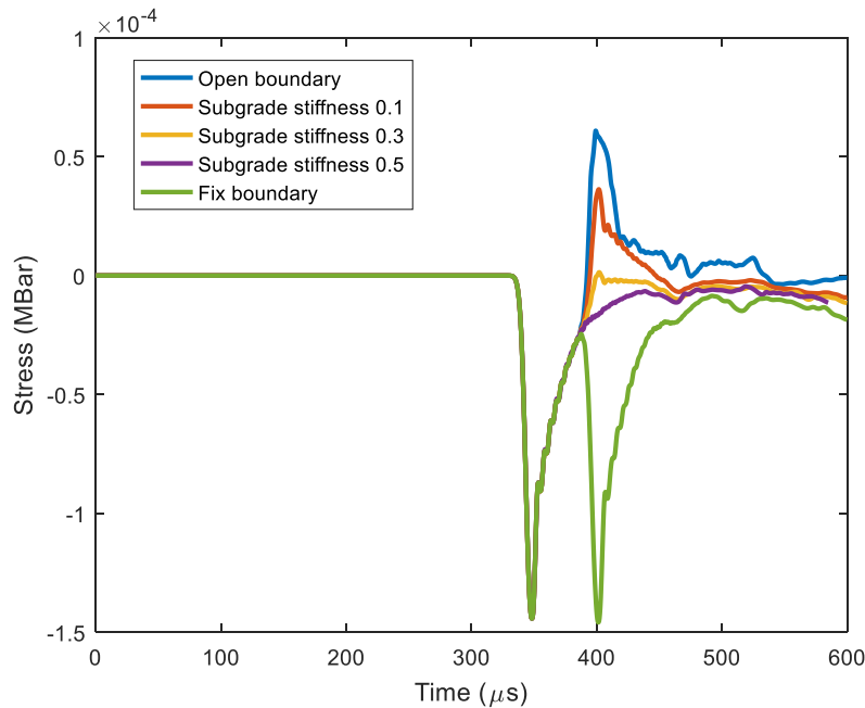
Figure 27: Stress comparison
