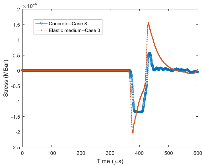
Figure 21: Stress comparison.
