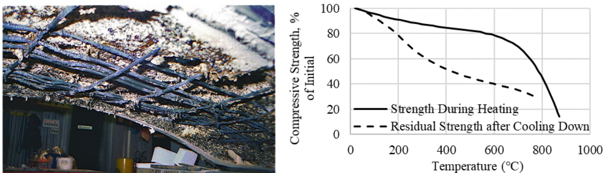
Figure 3: Typical concrete damage after heat exposure: spalling (Jansson 2013) (left) and strength reduction (ACI 2014) (right)
