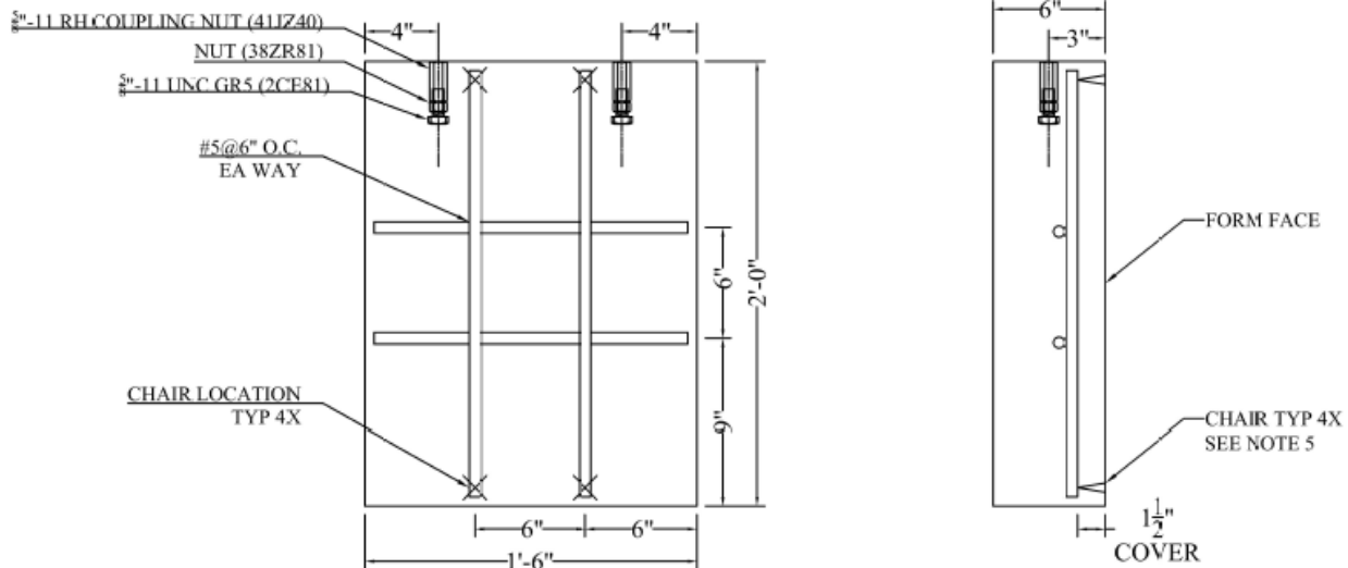
Figure 54: Concrete Specimen Detail (Typical)
